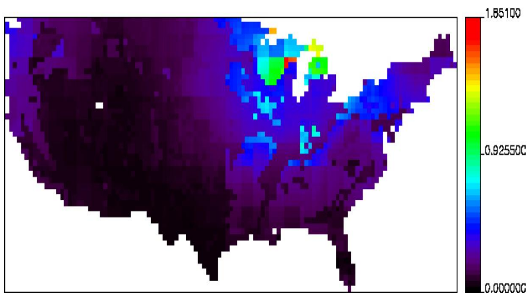
Figure 6 – Annual average dry \text{NO}_3 flux over the CONUS (kg N/ha/yr)
