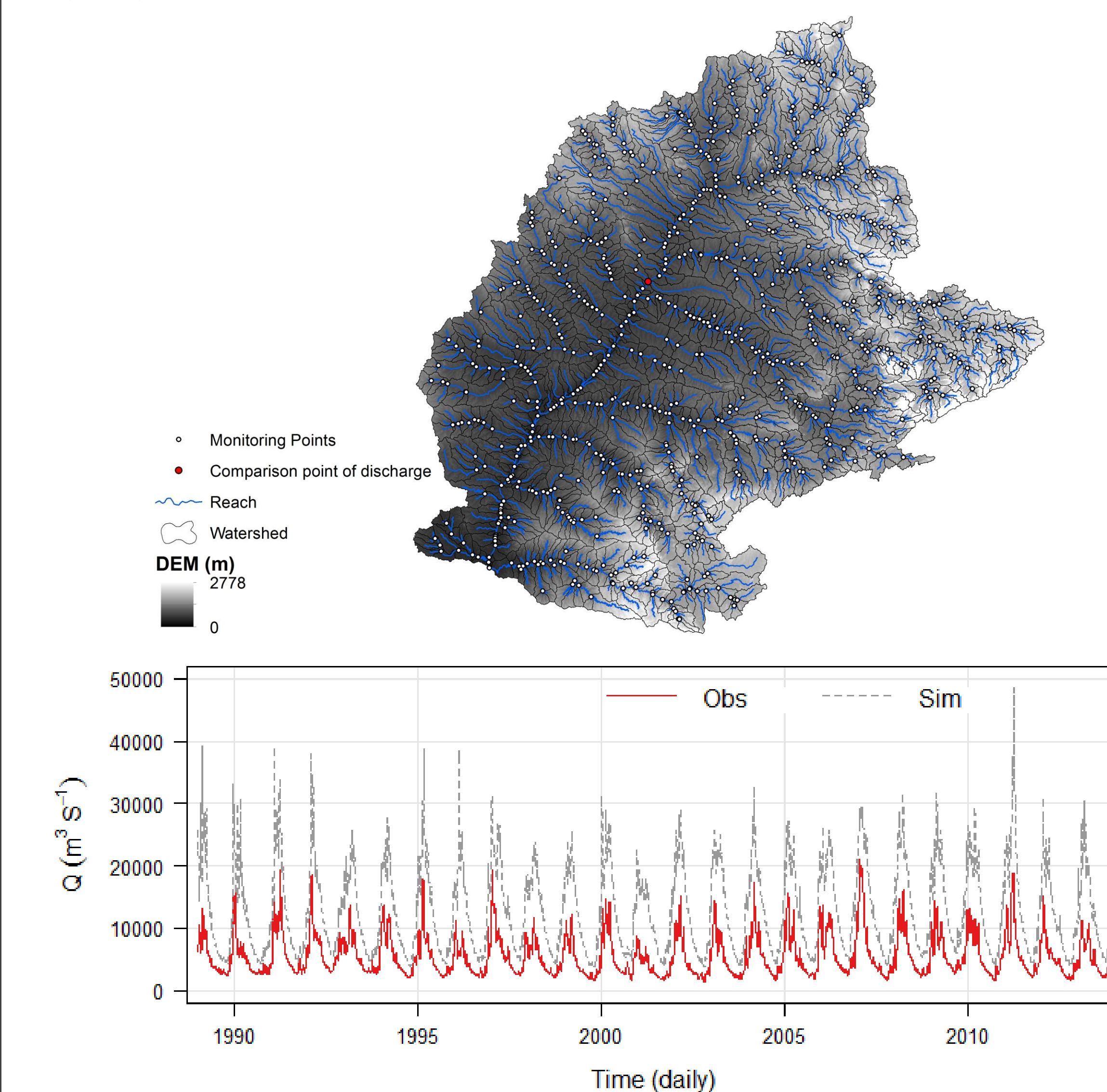
Figure 04. Sub-watersheds in the PRB domain and the comparison of simulated and observed daily outlet discharge located over Paraná river.
