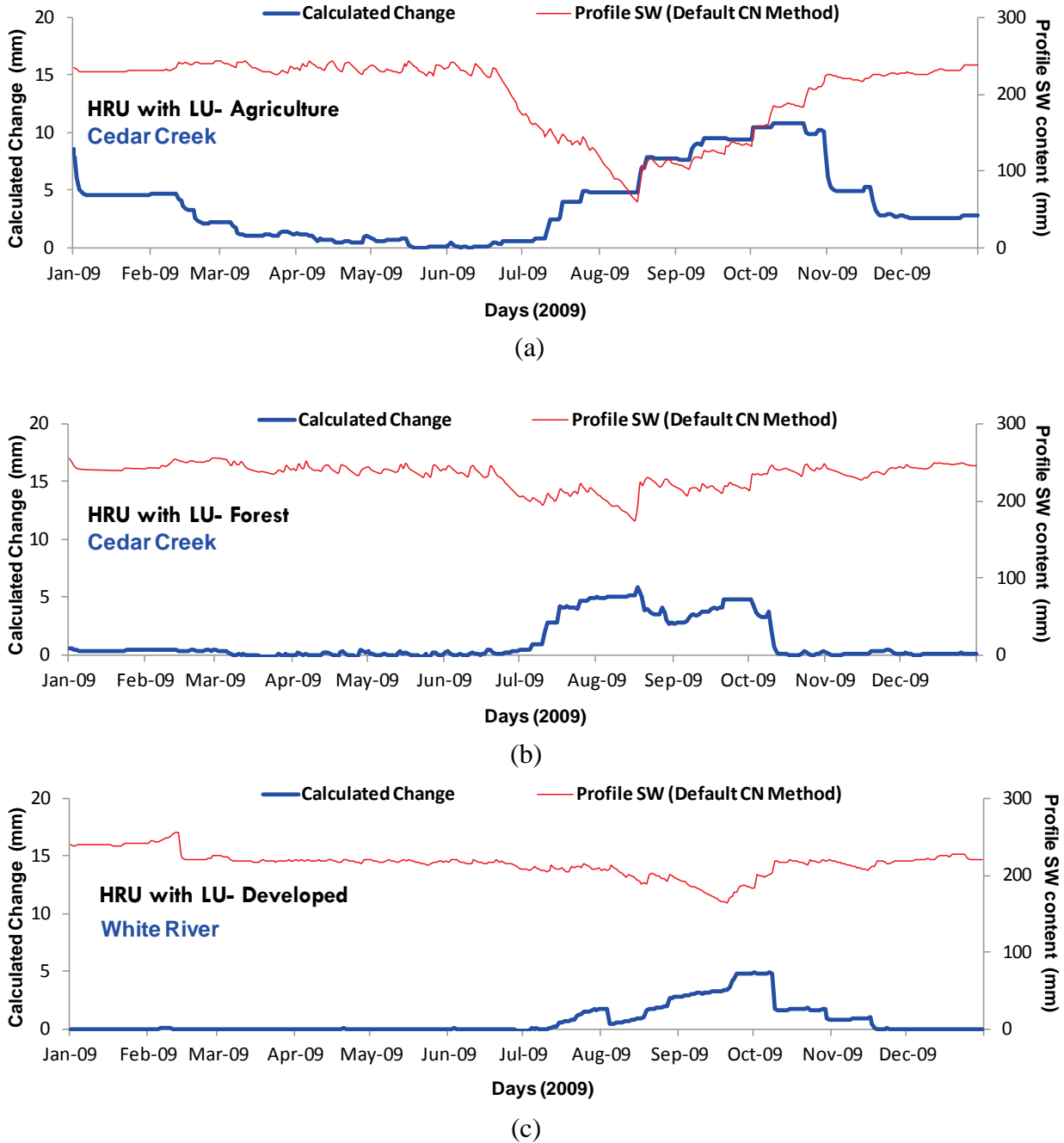
Figure 3. Area-weighted HRU-average soil profile water content with respective calculated difference (change = SMA method - Conventional Method): (a) agricultural landuse (Cedar Creek), (b) forested landuse (Cedar Creek), (c) developed landuse (White River). Patterns shown here are consistent in individual HRUs of particular LU types, as well as in watershed-scale.
