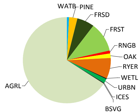
Figure 2. Share of Agricultural land in Black Sea Basin among other landuses, 65 %.
