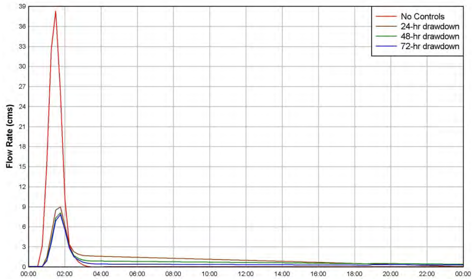
Figure 7. Hydrograph for Gilleland Tributary demonstrating the effects of varying drawdown time.
