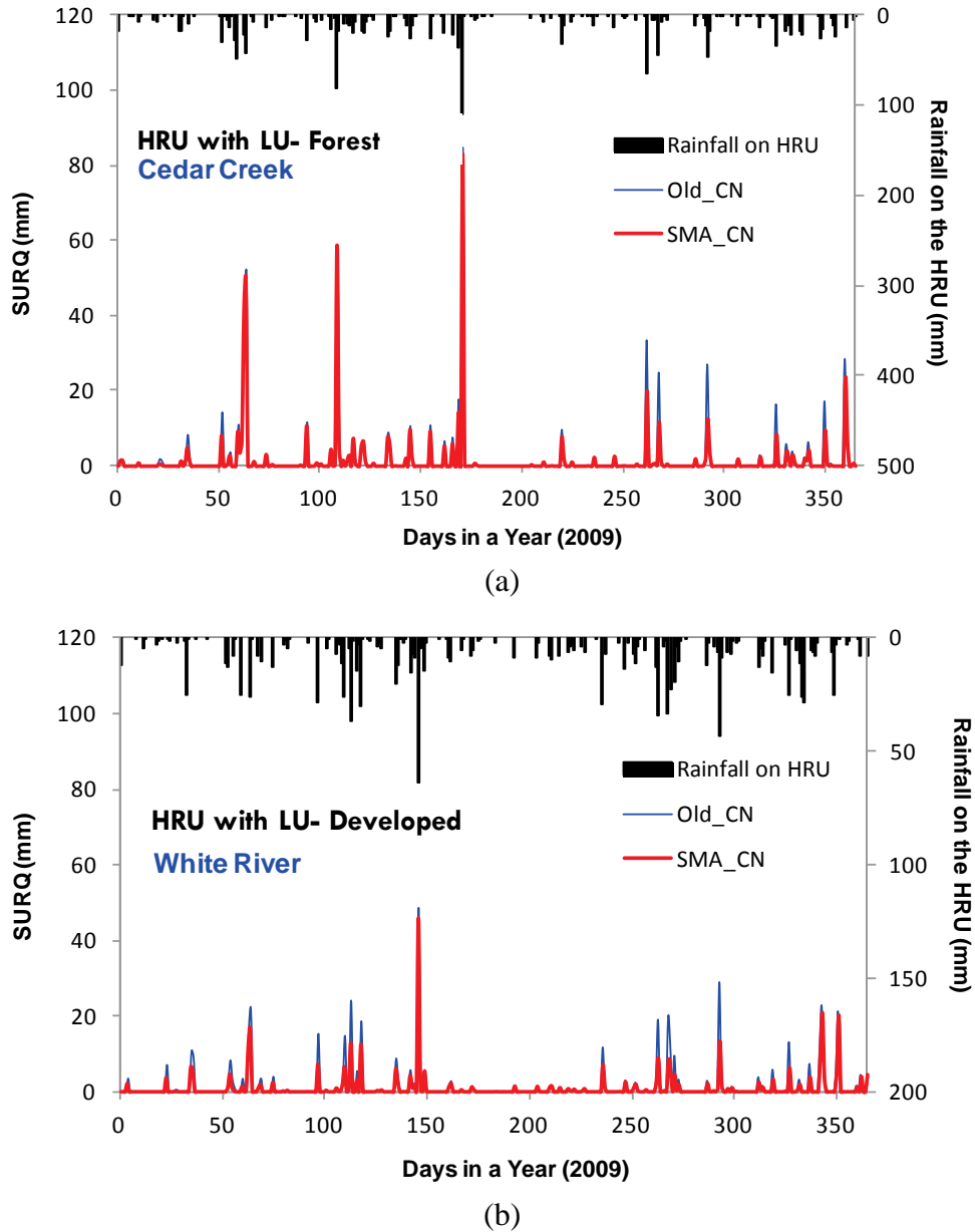
Figure 2. Comparison of uncalibrated HRU-level surface runoff between SMA and Original CN-based methods: (a) forested landuse (Cedar Creek), (b) developed landuse (White River).
