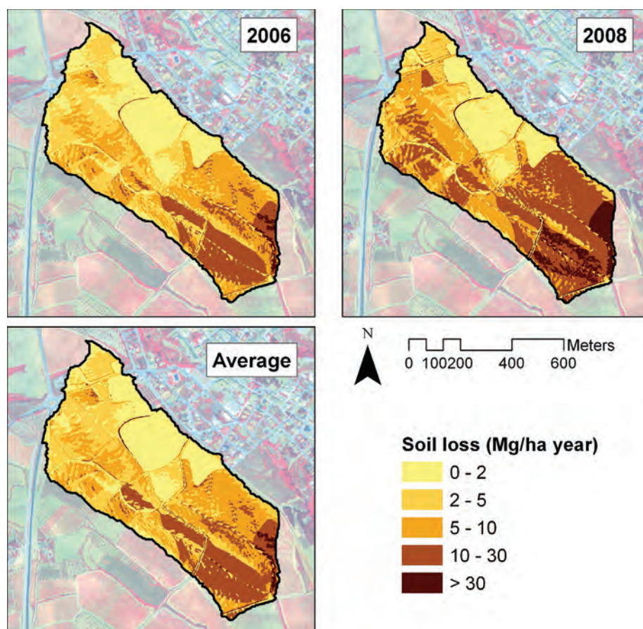
Figure 3. Average annual soil losses (2002-2012) and soil losses for two contrasted years: 2008 (very wet year) and 2006 (dry year).
