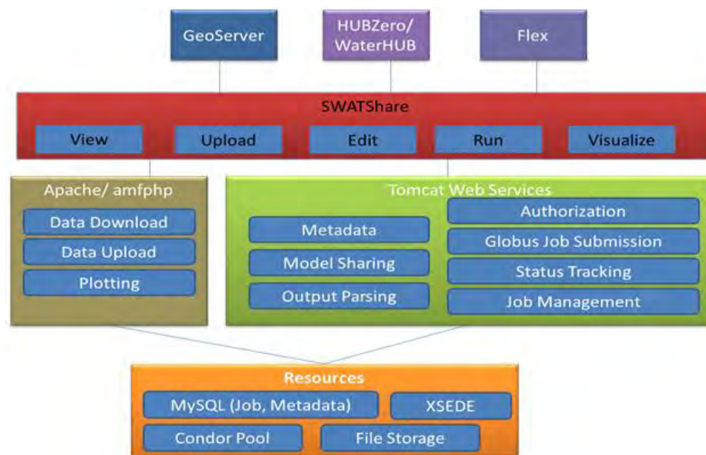
Figure 8. SWATShare Architecture
