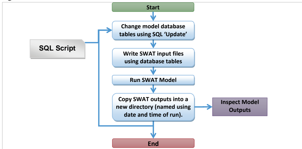
Figure 1: SWAT Model Automation
