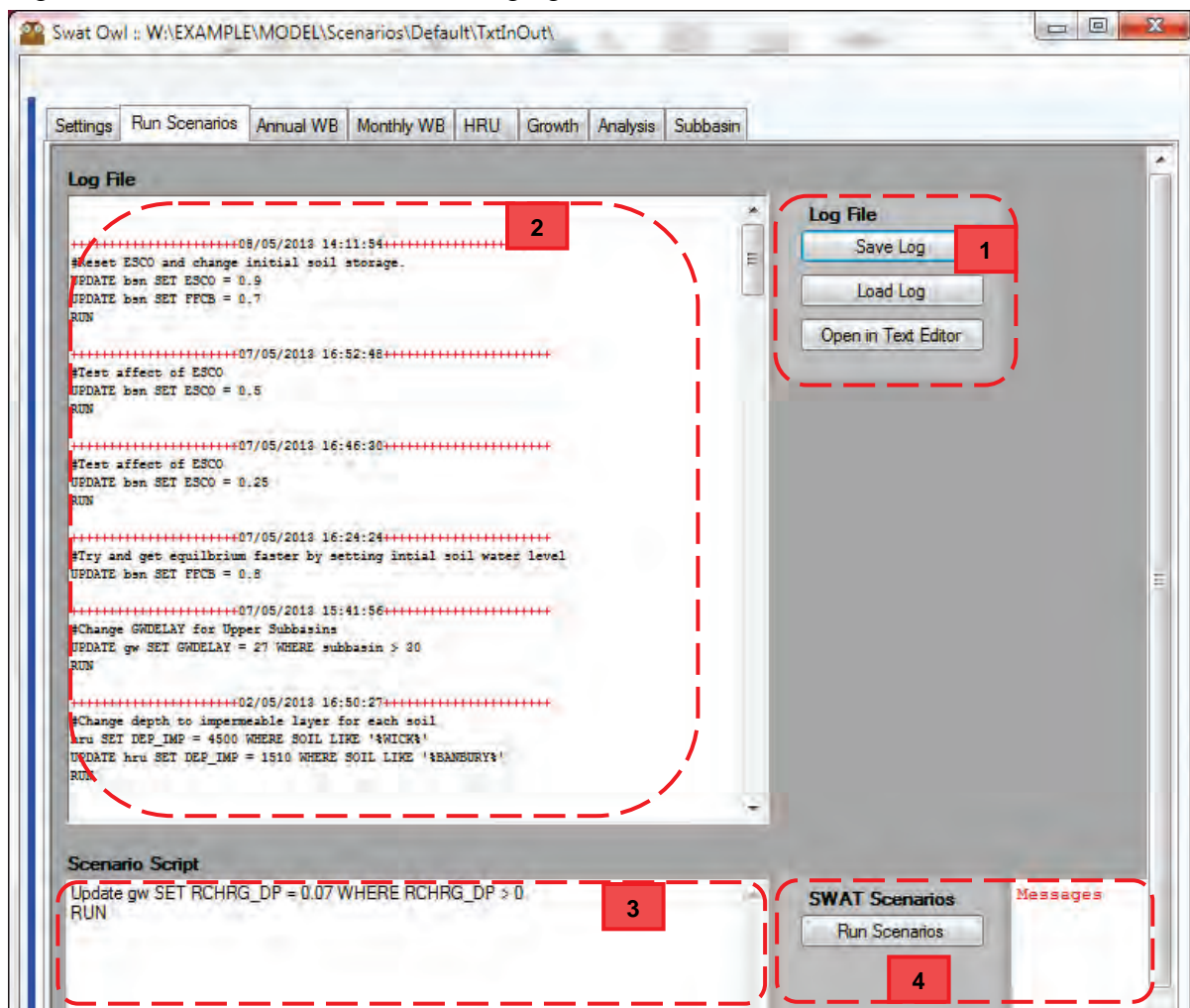
Figure A4: Automated Parameter Changing and Model Runs
