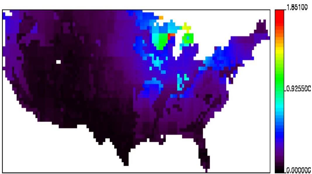
Figure 6 – Annual average dry NO 3 flux over the CONUS (kg N/ha/yr)
